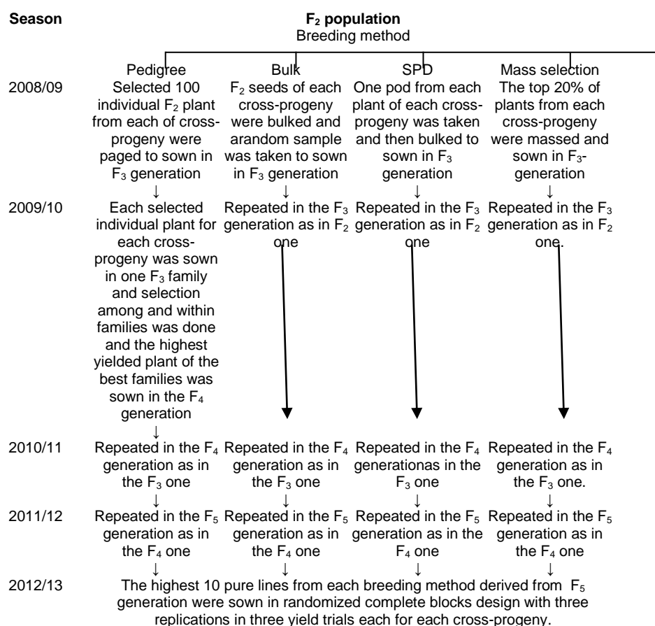
Fig. (1): Outline of generation advance for pedigree, mass selection, bulk and SPD breeding methods.
